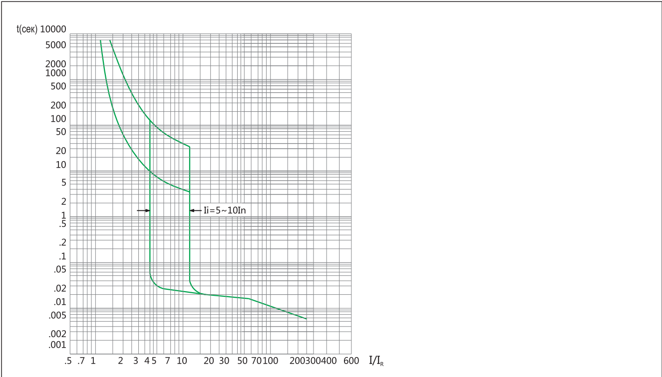
NM8-400,630(250A~,500A)
